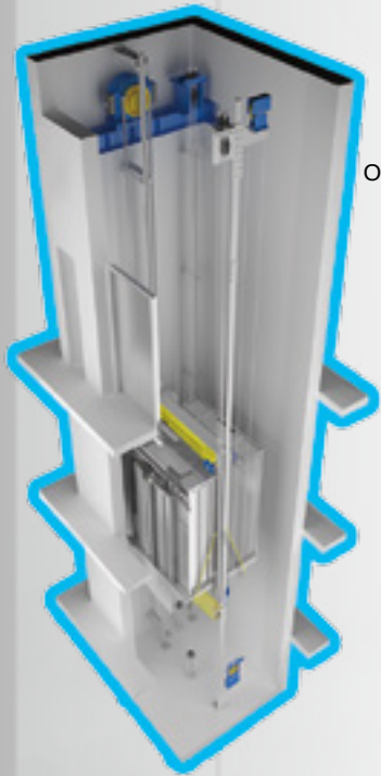
GEARLESS(VVVF)
