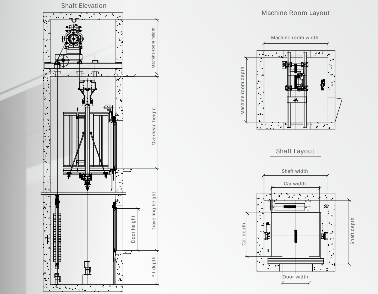
MR Passenger Elevator Technical Parameters
